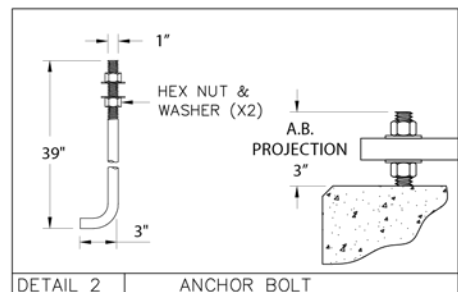
DETAIL 2 ANCHOR BOLT
