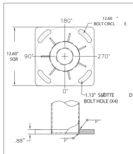
DETAIL 1 BASE PLATE
