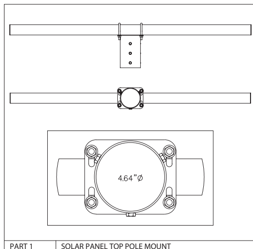
PART 1 SOLAR PANEL TOP POLE MOUNT
