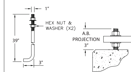
DETAIL 2 | ANCHOR BOLT
